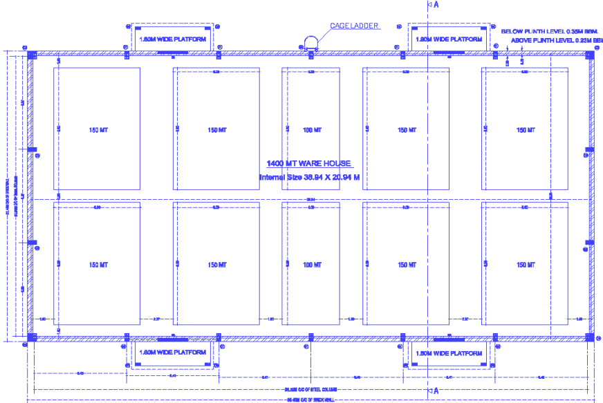
1400 MT WARE HOUSE UNIT PLAN
